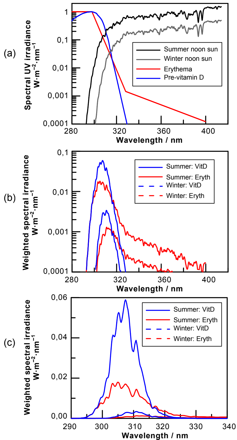
Figure 3 — a) Solar spectra measured at 45°S, during clear skies at noon close to the summer and winter solstices; also shown are the action spectra for erythema (ISO/CIE, 1999) and previtamin-D production (CIE, 2006)
