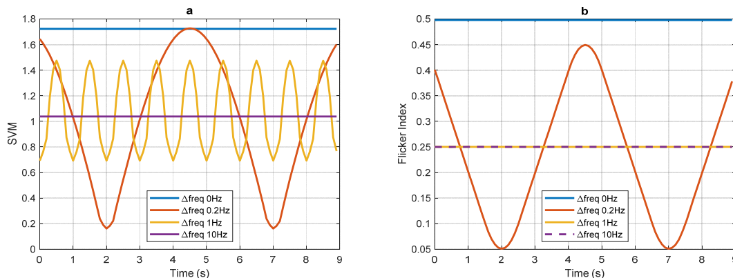
Figure 7 – Time resolved SVM (a) and FI (b) for two superposition square shaped waveforms at 500 Hz and 500+Δfreq Hz for four different Δfreq.
