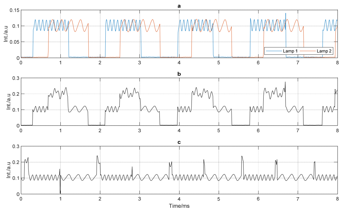
Figure 2 – a) Separated light intensity waveforms from lamp 1 @ 546.7 Hz and lamp 2 @ 551.8 Hz. b) Superposition of the two waveforms in a. c) Superposition of waveforms about 130 ms later compared to b.
